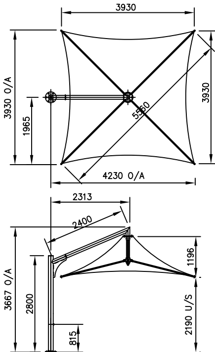
CODE: V40S VISTA 4.0M SQUARE CANTILEVER
