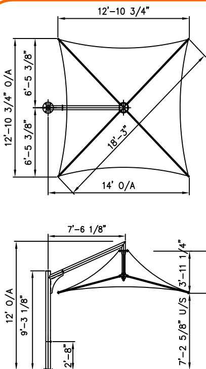
CODE: V40SC VISTA 14 FT. SQUARE CANTILEVER
